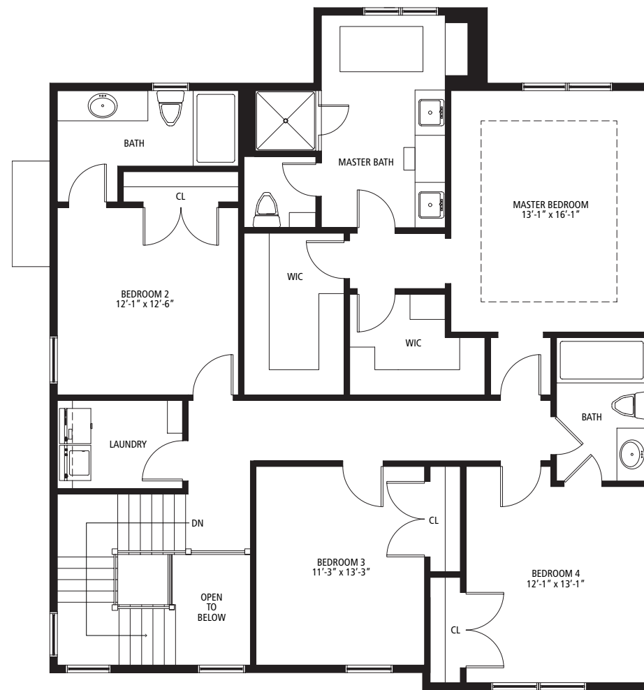
Second Floor
