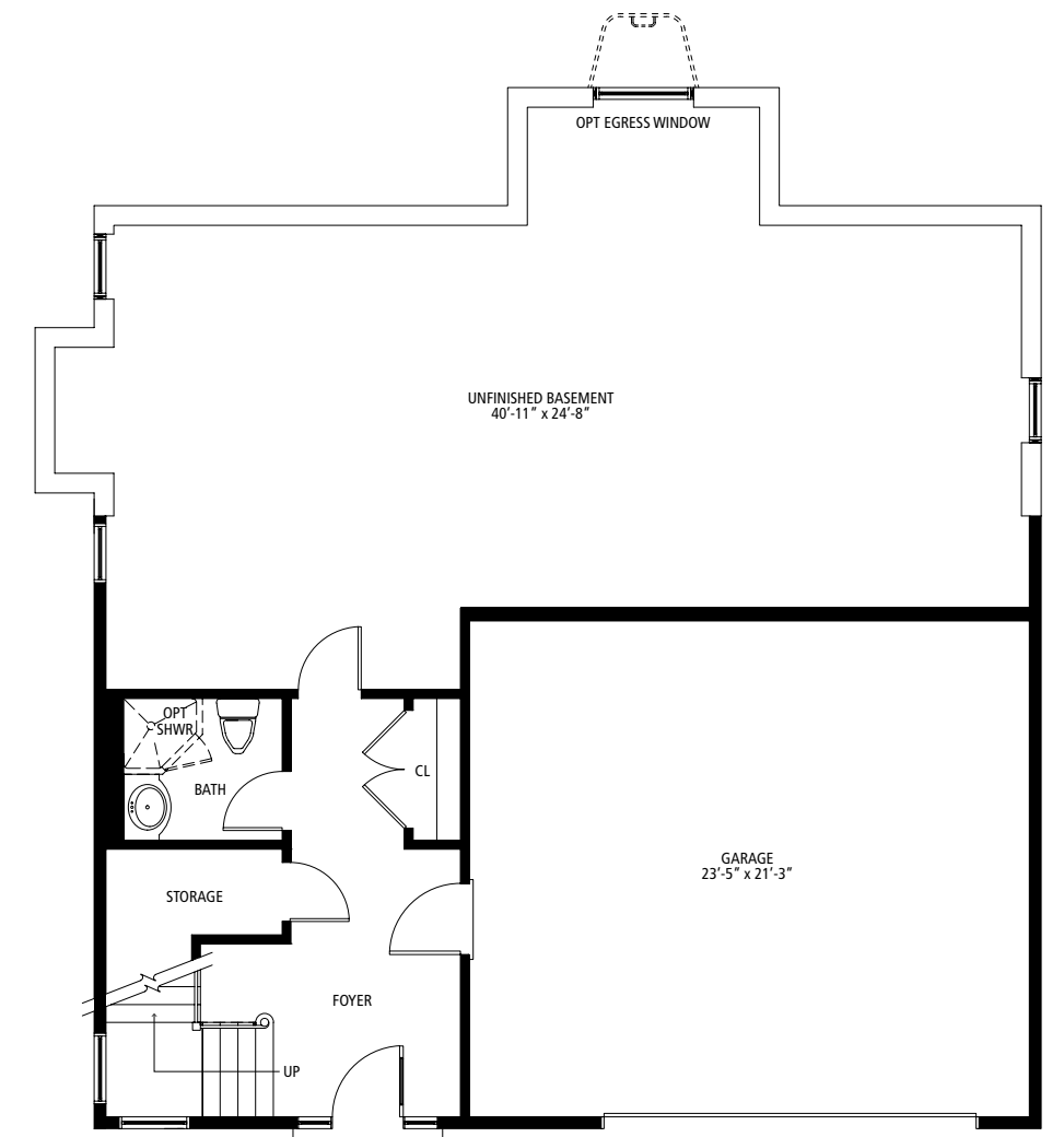
Basement
