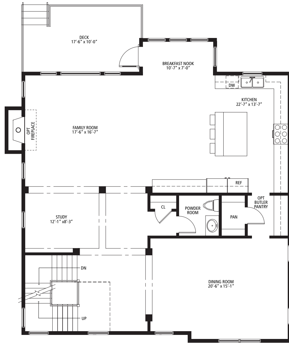
First Floor
