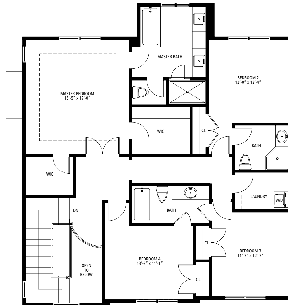
Second Floor
